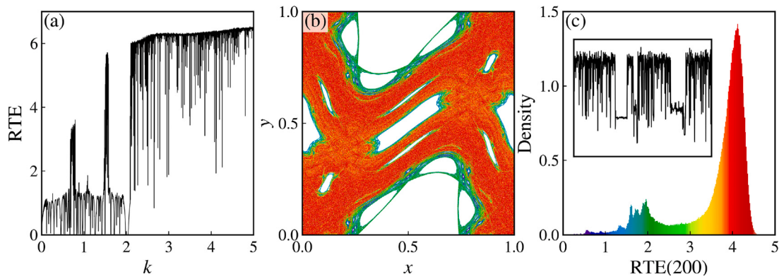
Fig. 9. (a) Demonstration of the use of the recurrence_time_entropy method of the DiscreteDynamicalSystem class of pymacsys to calculate the RTE as a function of the parameter k of the standard map [Eq. (1)] and (b) and (c) demonstration of the use the finite_time_recurrence_time_entropy method of the DiscreteDynamicalSystem class of pymacsys to calculate the distribution of finite-time RTE for the standard map with k = 1.5 . Execution times: (a) 19.2 s, (b) 804 ms, and (c) 35.2 s.
