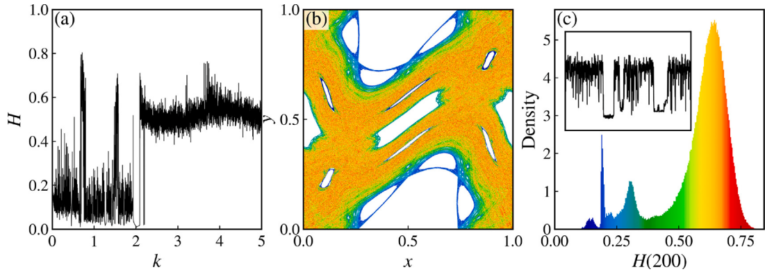
Fig. 10. (a) Demonstration of the use of the hurst_exponent method of the DiscreteDynamicalSystem class of pymcalsys to calculate the Hurst exponent as a function of the parameter k of the standard map [Eq. (1)] and (b) and (c) demonstration of the use the finite_time_hurst_exponent method of the DiscreteDynamicalSystem class of pymcalsys to calculate the distribution of finite-time H for the standard map with k = 1.5 . Execution times: (a) 1 min 9 s, (b) 2.78 s, and (c) 2 min 11 s.
