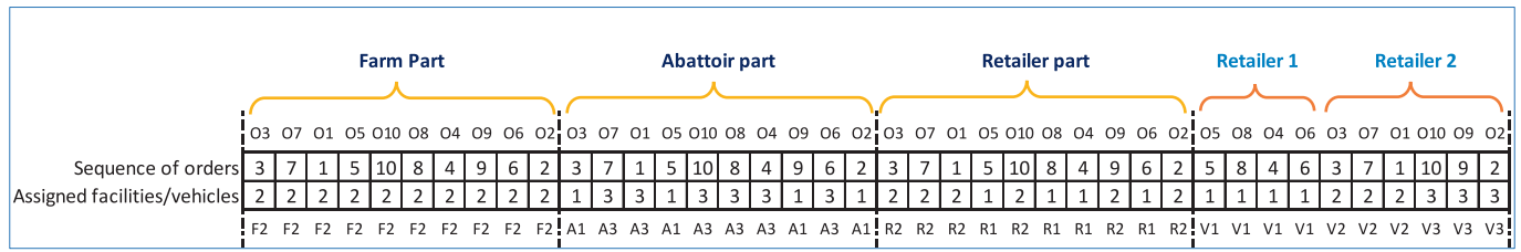
Fig. 2. Chromosome structure.
