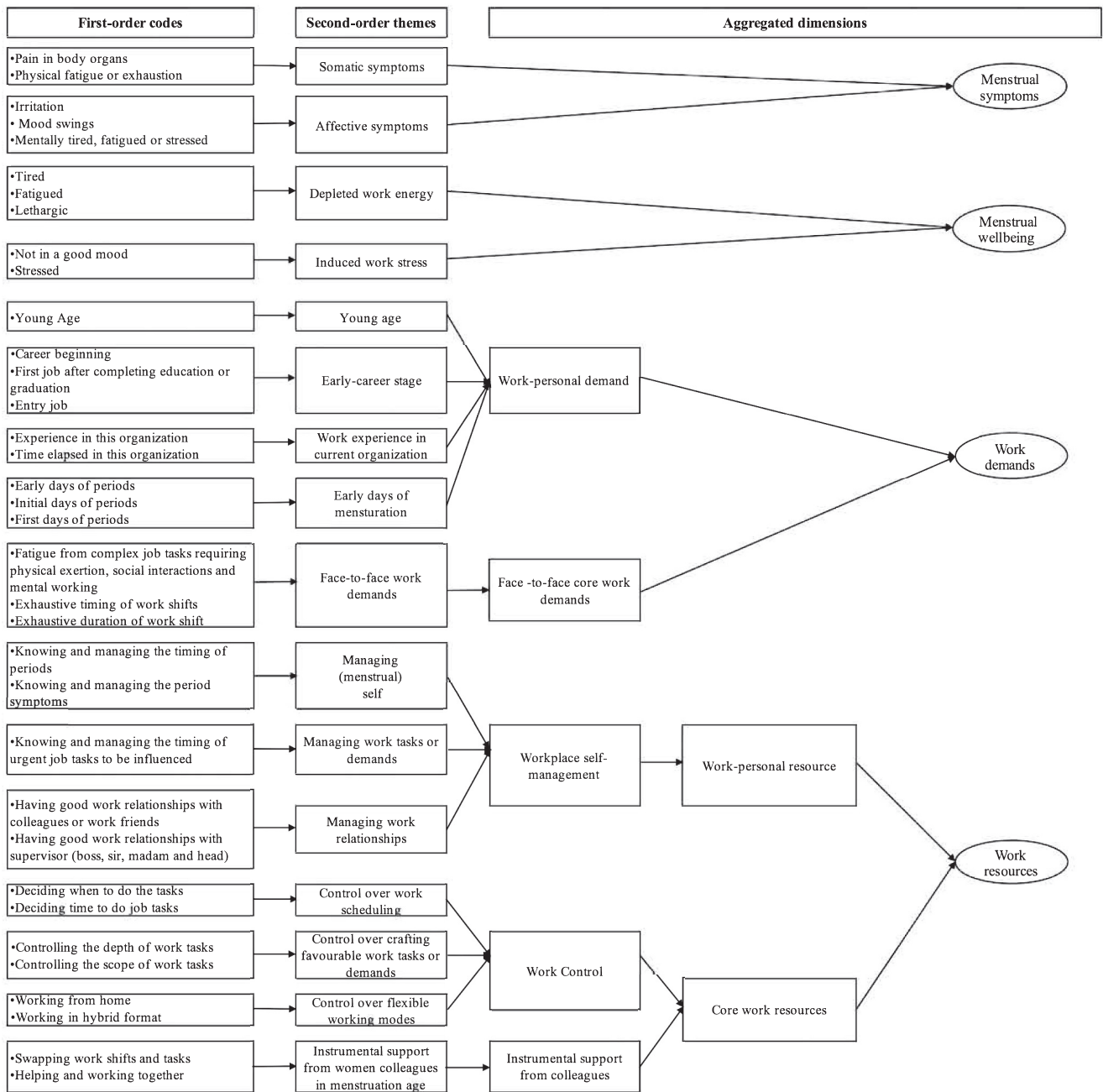
FIGURE 1 | Data structure.
