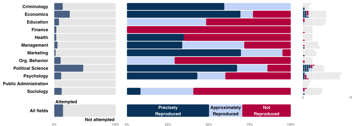
Figure S10. Reproducibility by 12 subfields and by year. Reproducibility as a percentage of the sample of papers from each year and each field.
