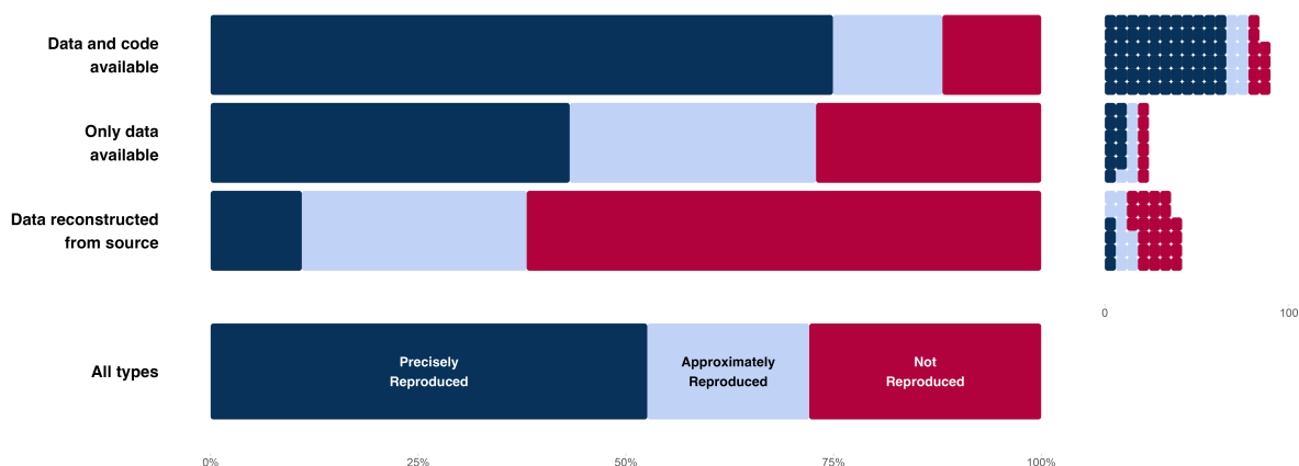
Figure 3. Reproducibility by data and code availability. Reproducibility as a percentage of attempts (left), and reproducibility as counts (right).
