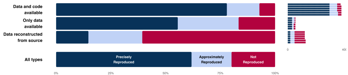
Figure S1. Reproducibility by whether data and code were available, only data were available, or when the paper's data were reconstructed from available source data for all claims. Reproducibility success rates as a percentage of attempts (left), and reproducibility success rates as counts (right).
