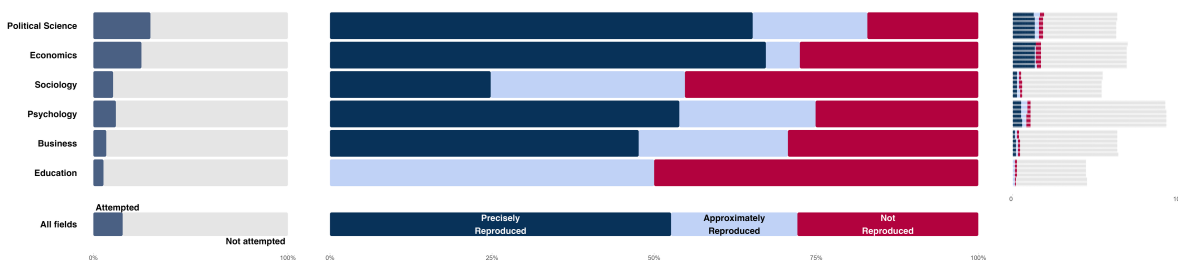
Figure S3. Reproducibility by field for all claims. The left column illustrates the proportion of outcome reproduction attempts from the sample of claims. The middle column illustrates reproducibility as a percentage of the attempts. The right column illustrates reproducibility as counts compared with the sample of claims.
