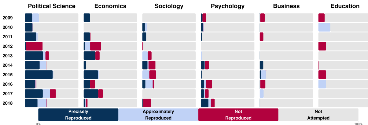
Figure S4. Reproducibility by field and year by paper as a proportion of the sample. Reproducibility as a percentage of the sample of papers from each year and each field.
