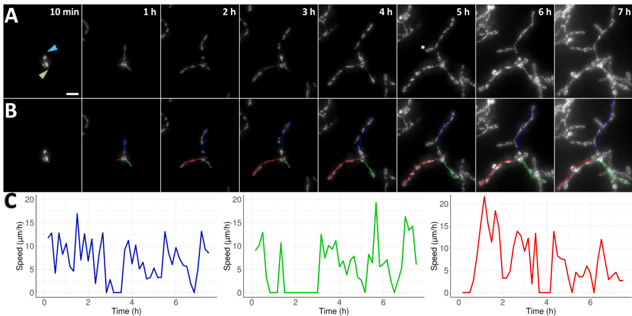
Fig. 1. (A) Greyscale images of Candida albicans in its initial unicellular yeast form, imaged at 60 \times magnification. Hyphae emerge from two cells (light blue and light green arrowheads) and continue to elongate over the course of seven hours. The top cell produces a single hypha, while the bottom cell produces two hyphae at opposite poles. At five hours (5 h), a secondary hypha (white asterisk) emerges from the primary hypha. Scalebar 10 \mu\text{m} . (B) Paths of the emerging primary hyphae are shown (blue, green and red). (C) Graphs of hyphal speeds over seven hours, with colours corresponding to the hyphal tracks shown in B). Hyphal growth is intermittent, with phases of zero hyphal elongation. (For interpretation of the references to colour in this figure legend, the reader is referred to the web version of this article.)
