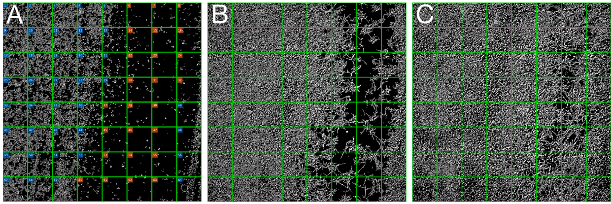
Fig. 5. Biofilm scratch assay. (A) Initial condition. The FOV imaged at 15× magnification partitioned into 64 squares. High-density, blue markers. Low-density, orange markers. Coverage of basal well surface after (B) 6 h and (C) 12 h. Each partitioned square covers 132 \mu\text{m} \times 132 \mu\text{m} . (For interpretation of the references to colour in this figure legend, the reader is referred to the web version of this article.)
