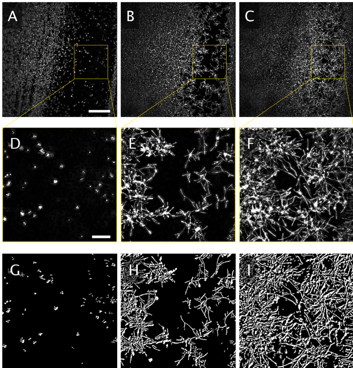
Fig. 4. Large FOV at low resolution showing (A) biofilm initiation at single cell stage with scalebar 200 \mu\text{m} , (B) biofilm development after 6 h and (C) after 12 h. (D) to (F) are the magnified insets of the yellow squares in (A) to (C), respectively, with a scalebar of 50 \mu\text{m} . (G) to (I) are the corresponding binary images. (For interpretation of the references to colour in this figure legend, the reader is referred to the web version of this article.)
