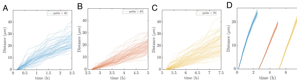
Fig. 2. Automated tracking of multiple hyphae in three time windows of 2.5 h length each. (A) to (C) Hyphal path distance with time. (A) 0–2.5 h, 48 hyphae. (B) 2.5–5 h, 63 hyphae. (C) 5–7.5 h, 70 hyphae. D) The time windows from A to C are concatenated in one graph and shown as average distance ( \mu\text{m} ) over time. The semi-transparent region around each solid curve for the mean represents the 95% CI.
