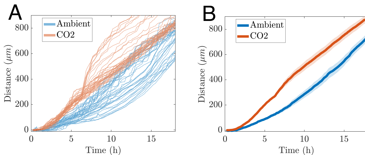
Fig. 8. Time evolution of mature biofilm front in direction perpendicular to basal well surface. Ambient conditions, blue. Elevated \text{CO}_2 levels, red. (A) Displacement of individual equally partitioned regions of the front. (B) Average displacement of front (solid curves) with the semi-transparent region indicating the 95% CI. (For interpretation of the references to colour in this figure legend, the reader is referred to the web version of this article.)
