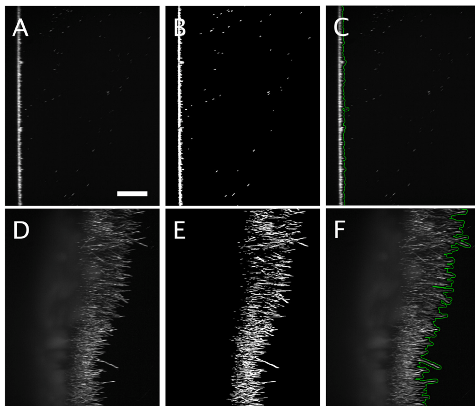
Fig. 7. Vertical expansion of a C. albicans biofilm using LSM. The top row shows images at the time point 0, the bottom row shows images after 18 h of growth. (A, D) Original images. (B, E) Binarised images after thresholding. (C, F) Processed images showing the biofilm front (green curves) of growing hyphae. Scalebar 200 \mu\text{m} . (For interpretation of the references to colour in this figure legend, the reader is referred to the web version of this article.)
