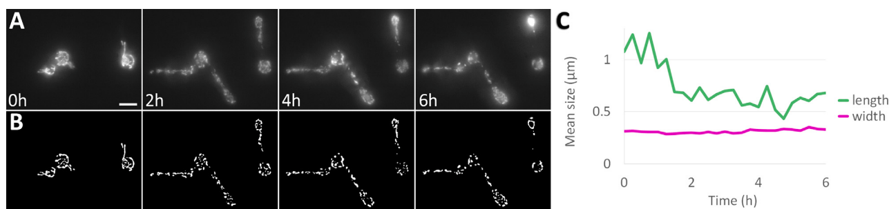
Fig. 3. Mitochondrial fragmentation indicates phototoxicity at high magnification. (A) Fluorescently labelled mitochondria show hyphal emergence from single cells at 150× magnification over six hours. Scalebar 5 μm. (B) Processed images showing the isolated mitochondria. (C) Quantification showing mitochondrial fragmentation. The average length (green) of mitochondria is greatly reduced after two hours, while their width (magenta) remains unchanged. (For interpretation of the references to colour in this figure legend, the reader is referred to the web version of this article.)
