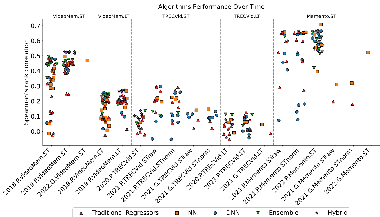
Fig. 9 Analysis of the employed methods for all the prediction and generalisation subtasks. We plot Spearman's rank correlation for all methods.
