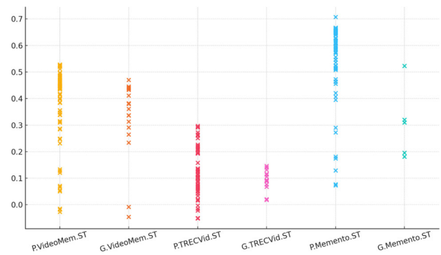
Fig. 10 Performance comparison between the prediction (P) and generalisation (G) challenges on the VideoMem.ST, TRECvid.ST, and Memento.ST datasets.
