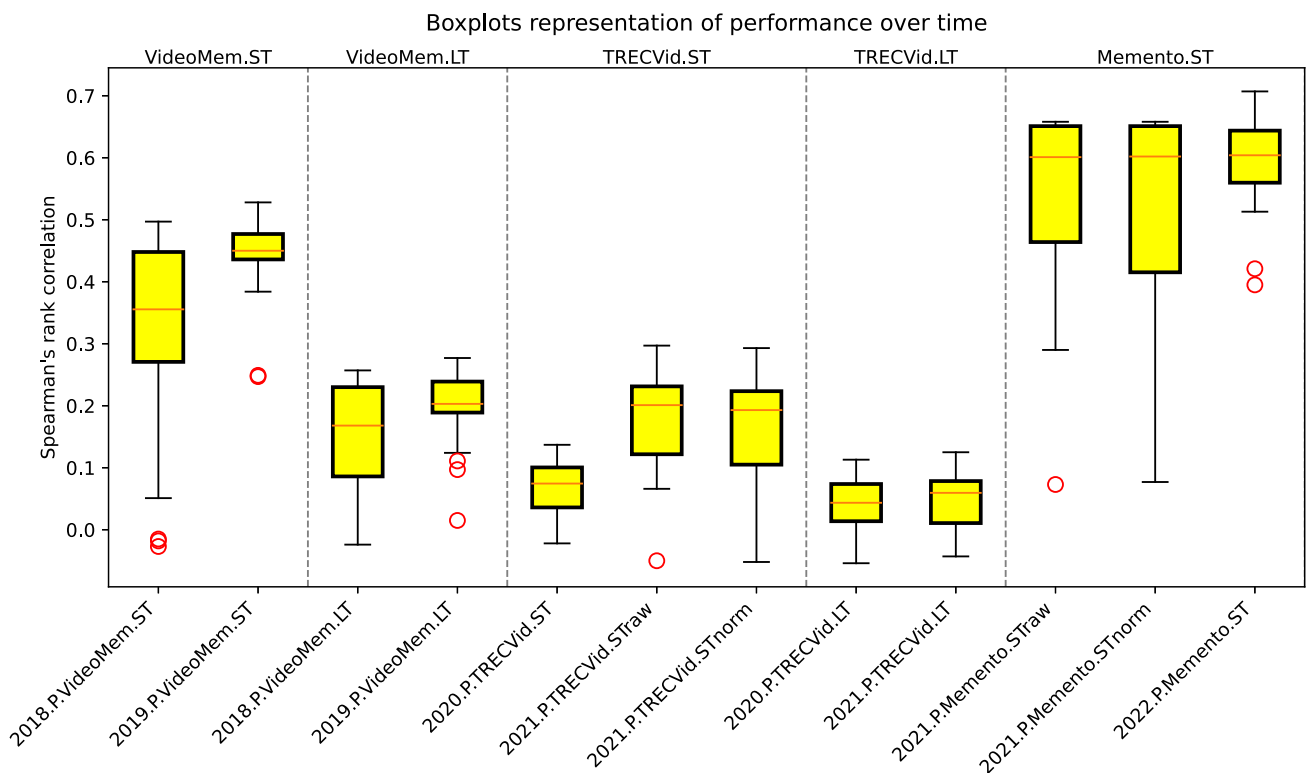
Fig. 7 Boxplot representation of the overall performance of methods across various versions of the dataset, for the prediction challenge. We use the following parameters in creating the boxplot representation: interquartile range IQR = 50\% , median values represented by the red
