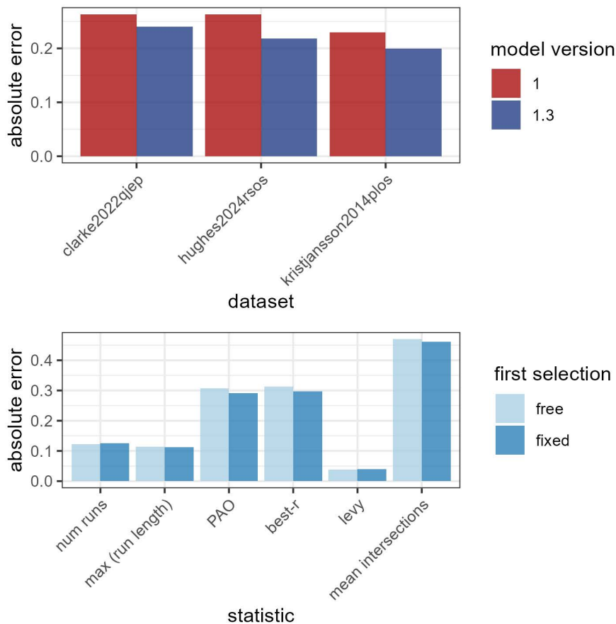
Fig 11. (top): estimate of scaled absolute error averaged across first selection variants and statistics, for each dataset and model version. (bottom): estimate of scaled absolute error averaged across datasets for model v1.3, for fixed and free first selection and for each statistic.
