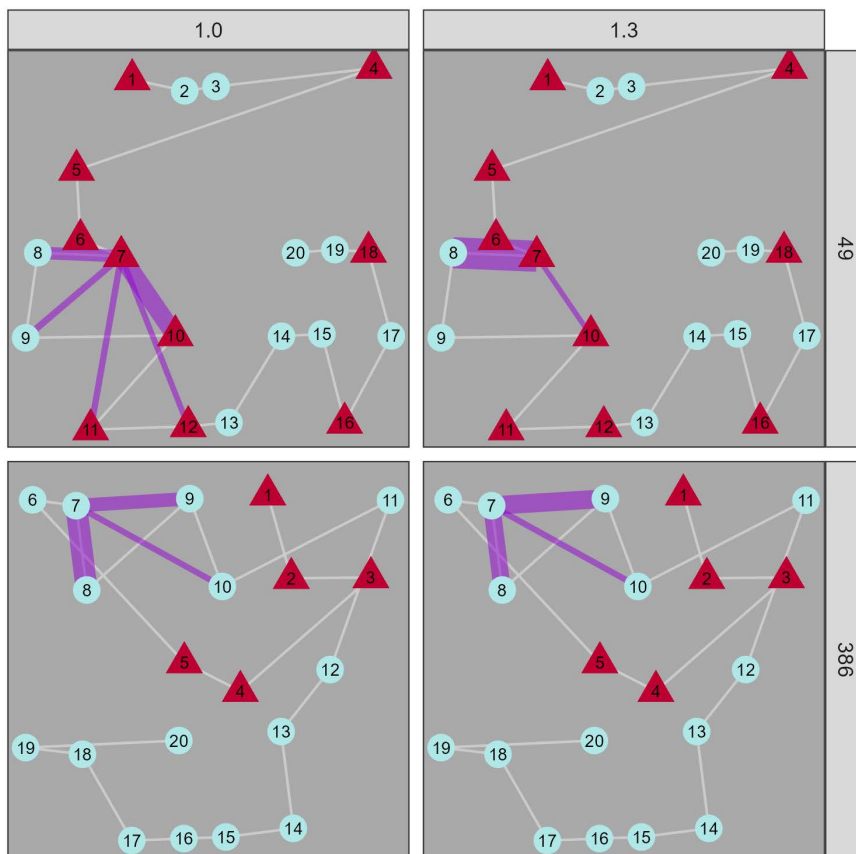
Fig 8. Comparison of simulated paths from FoMo v1.0 and v1.3 with observed data from a human participant from the [74] dataset. The items are illustrated as red triangle and pale blue circles, and the white line illustrates the order in which the human participant selected the items. The purple lines indicate the weightings that the model assigns to each possible next target (thicker means more weight).
