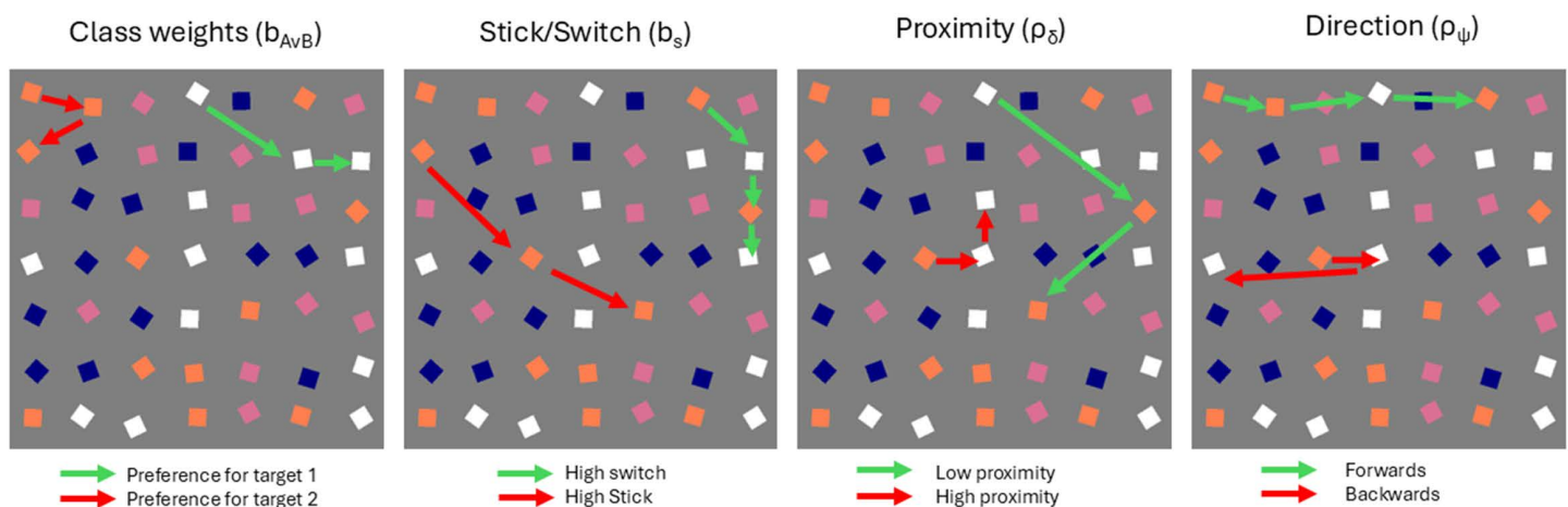
Fig 3. The original [7] model parameters. From left to right: stick/switch rate, class weights, proximity tuning, and direction tuning.
