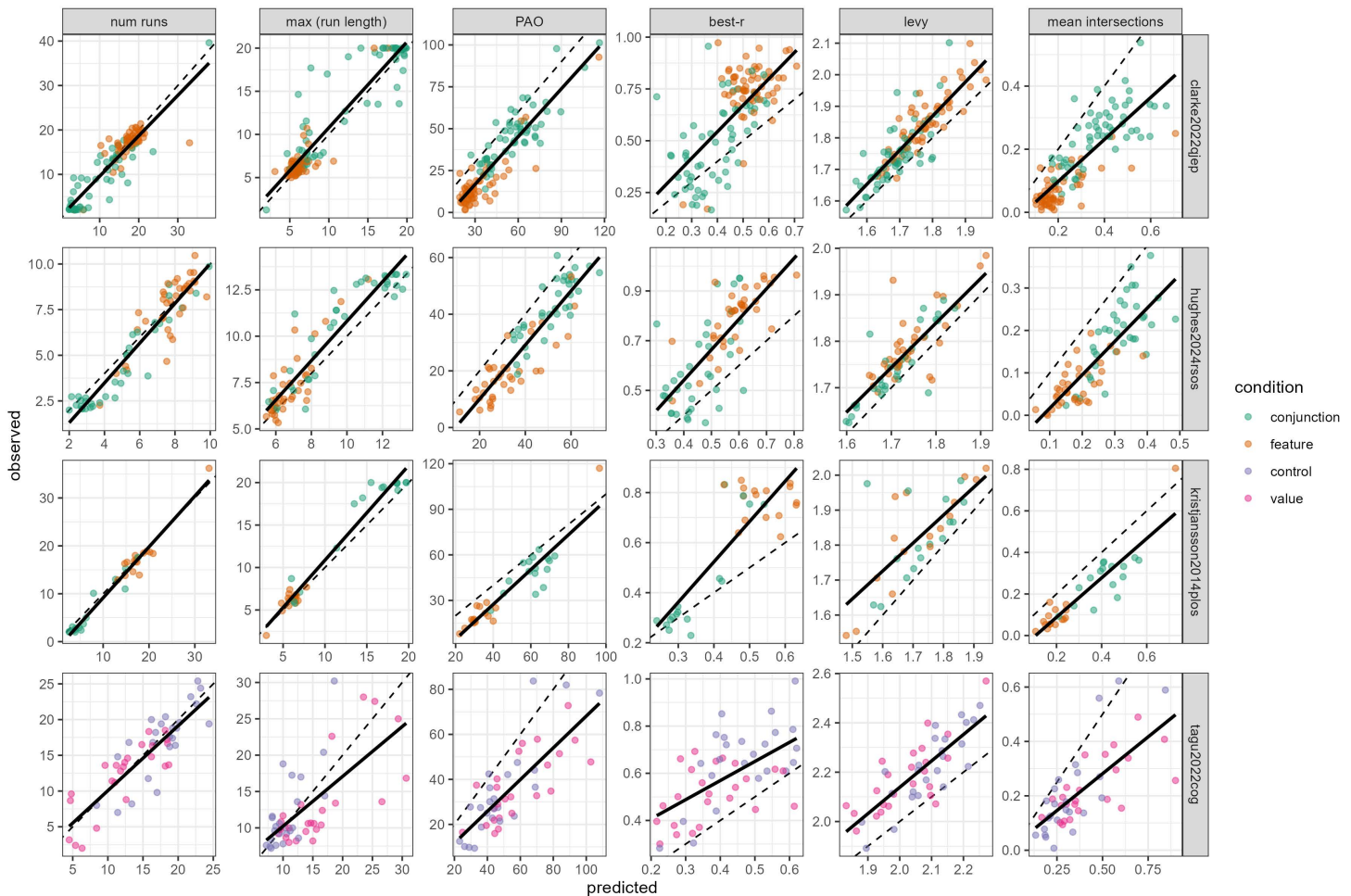
Fig 9. Comparison of predicted and observed path statistics (FoMo v1.3) over a range of datasets. Each dot represents an individual participant in a condition, the dotted line indicates the y=x identity line, while the solid black lines give the best fit linear regression. Note that the poorer performance for the [73] is almost certainly due (at least in part) to our use of an exhaustive foraging model to account for an inexhaustive paradigm.
