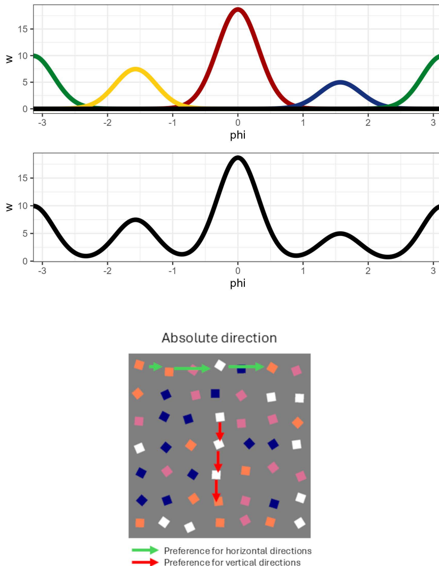
Fig 4. (top): Illustration of four von Mises distributions (top) that can be summed to give (middle) a multi-model distribution that is able to flexibly weight horizontal and vertical directions. (bottom): How these weights could encode different strategies.
