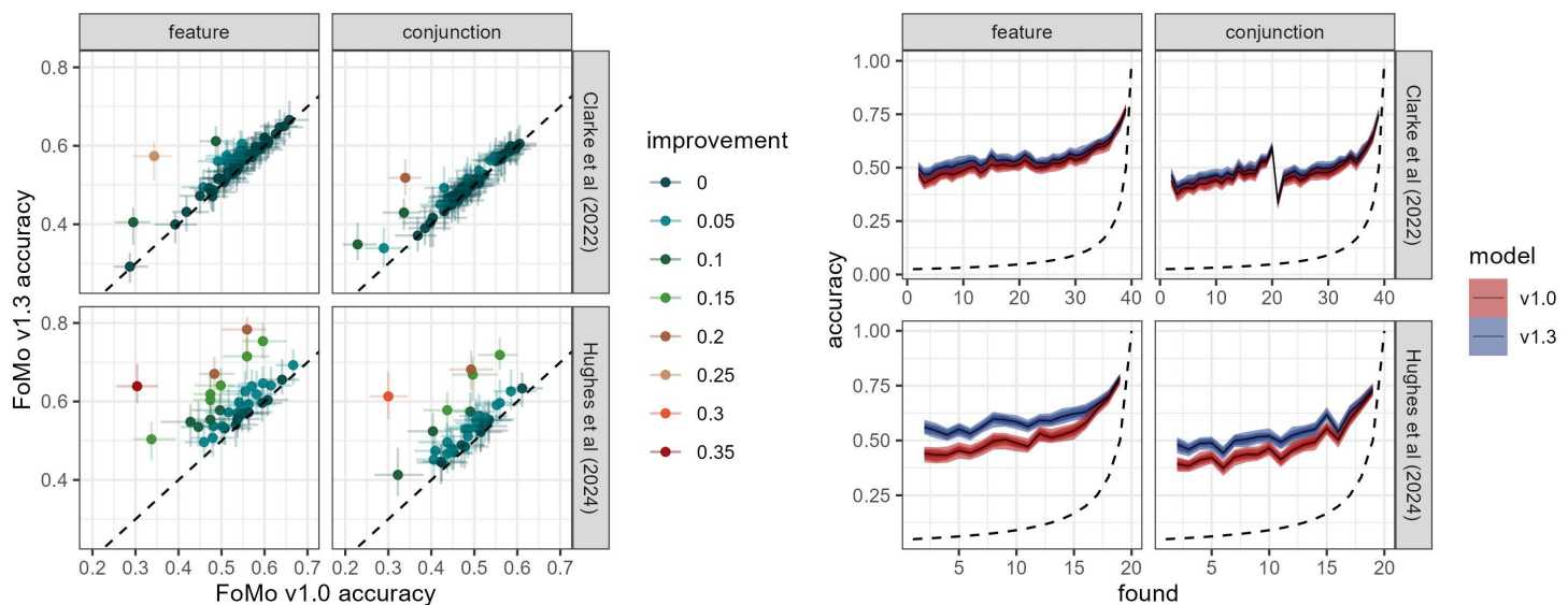
Fig 6. (left): Comparison in accuracy between FoMo v1.0 and 1.3 for the [42] and [74] data. Each point represents an individual participant, and the crosshairs provide the 95% Highest Posterior Density Interval (HPDI). Colours indicate the improvement in accuracy between models. (right): 95% HPDI for accuracy throughout a trial for FoMo v1.3. The dotted line indicates chance performance.
