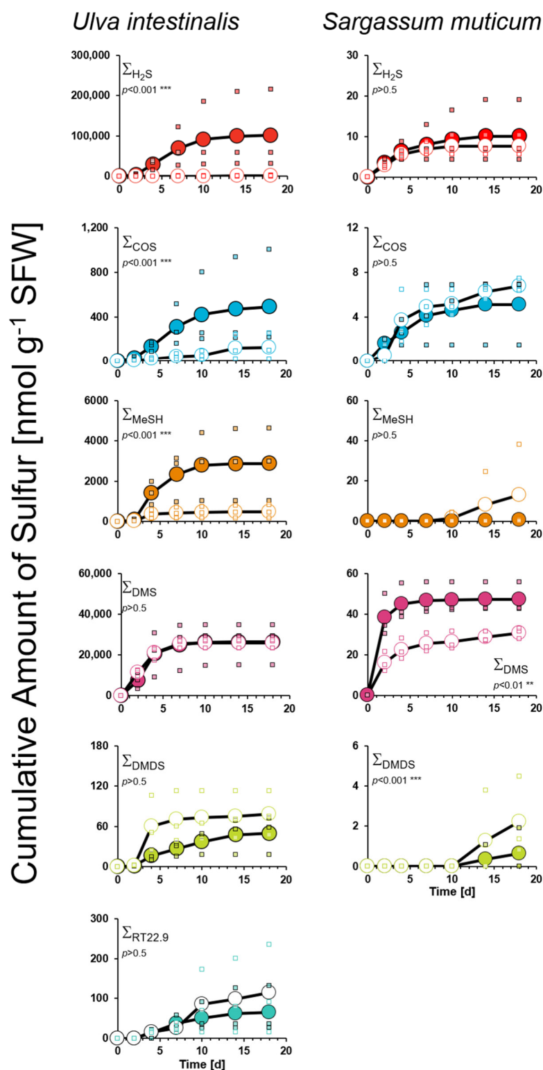
Figure 1. Cumulative amount of volatile sulfur released from decaying seaweed. Hypoxic incubations with Ulva intestinalis (left) and Sargassum muticum (right) at 26 °C for 18 d. Shown are mean values after incubation in seawater (SW; closed circles) or freshwater (FW; open circles). Data were normalised to seaweed freshweight (SFW) biomass with biological triplicates presented using squared symbols (RT22.9 = unidentified sulfur volatile). Please note variable scaling along the y-axes. Asterisks and associated p -values indicate the level of statistical difference between SW and FW treatments.
