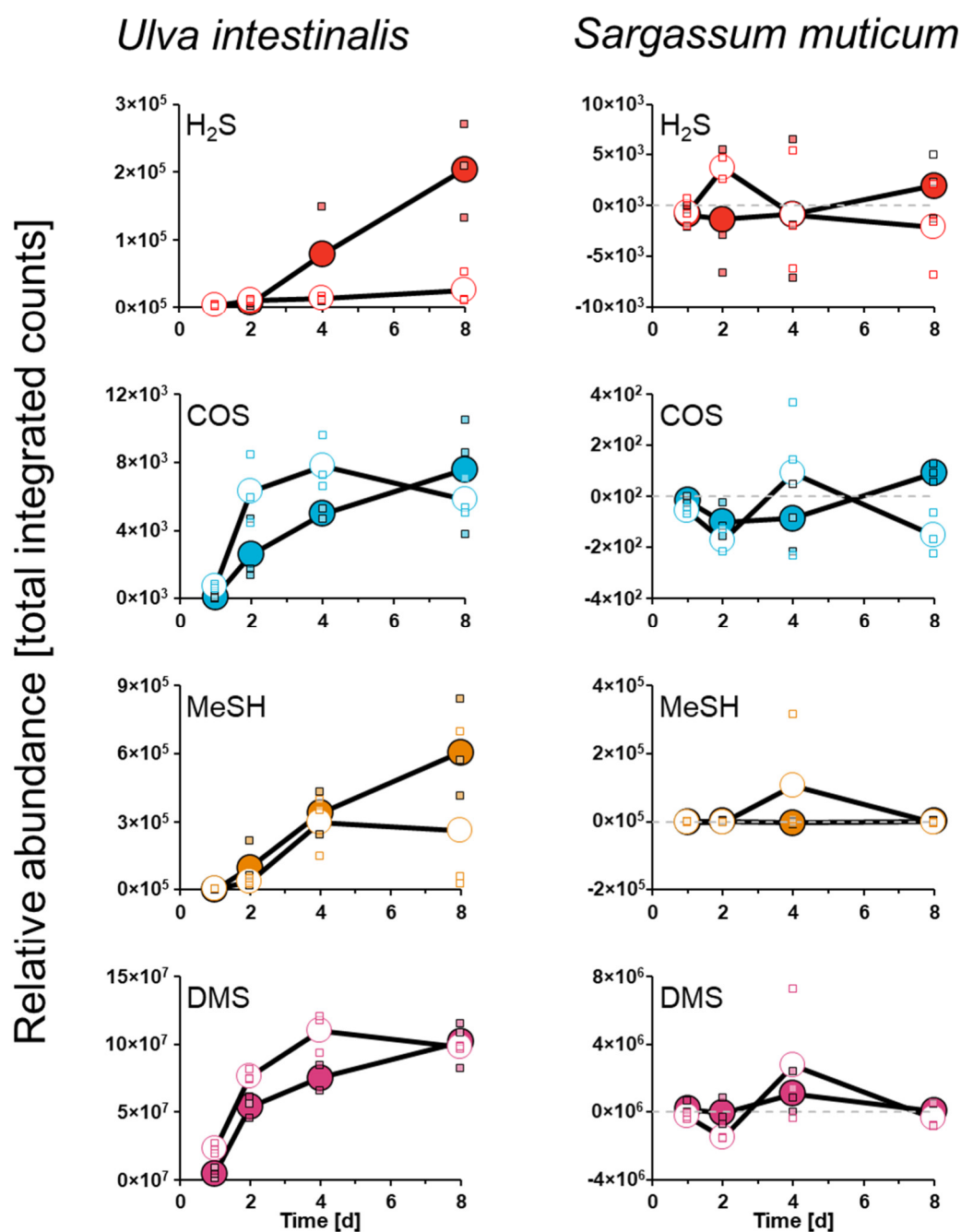
Supplementary Figure S2. PTR-MS qualitative assessment of sulfur gases produced by decaying Ulva intestinalis and Sargassum muticum . Hypoxic incubations with Ulva intestinalis (left) and Sargassum muticum (right) at 26 °C for 8 d. Shown are mean relative abundances after incubation in seawater (SW; closed circles) or freshwater (FW; open circles) with biological triplicates presented using squared symbols (except n = 2 for seawater incubation with U. intestinalis on day 4 due to failure of gas-tight seal in one of the vials, and freshwater incubation with S. muticum on day 2 due to file corruption). Please note variable scaling along the y-axes with dashed line in S. muticum panels indicating zero.
