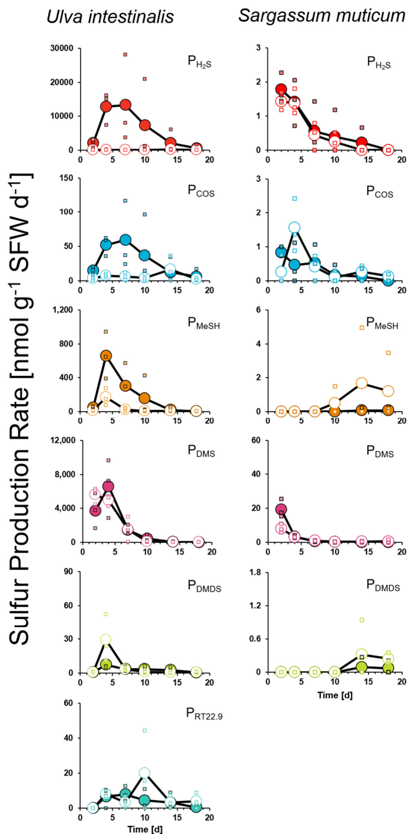
Figure 2. Net-production rate of volatile sulfur released from decaying seaweed. Hypoxic incubations with Ulva intestinalis (left) and Sargassum muticum (right) at 26 °C for 18 d. Shown are mean values after incubation in seawater (SW; closed circles) or freshwater (FW; open circles). Data were normalised to seaweed freshweight (SFW) biomass with biological triplicates presented using squared symbols (RT22.9 = unidentified sulfur volatile).
