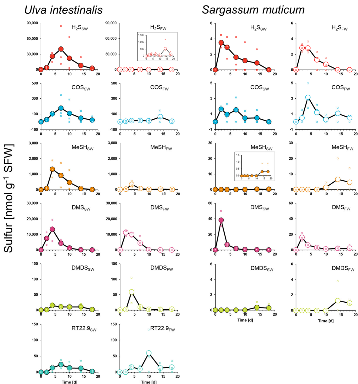
Supplementary Figure S3. Gas-chromatographic quantification of volatile sulfur released from decaying Ulva intestinalis and Sargassum muticum . Hypoxic incubations with Ulva intestinalis (left) and Sargassum muticum (right) at 26 °C for 18 d. Shown are mean values after incubation in seawater (SW; closed circles) or freshwater (FW; open circles). Data were normalised to seaweed freshweight (SFW) biomass with biological triplicates presented using squared symbols (RT22.9 = unidentified sulfur volatile). Inserts for H 2 S and MeSH present detail. Please note variable scaling along the y-axes.
