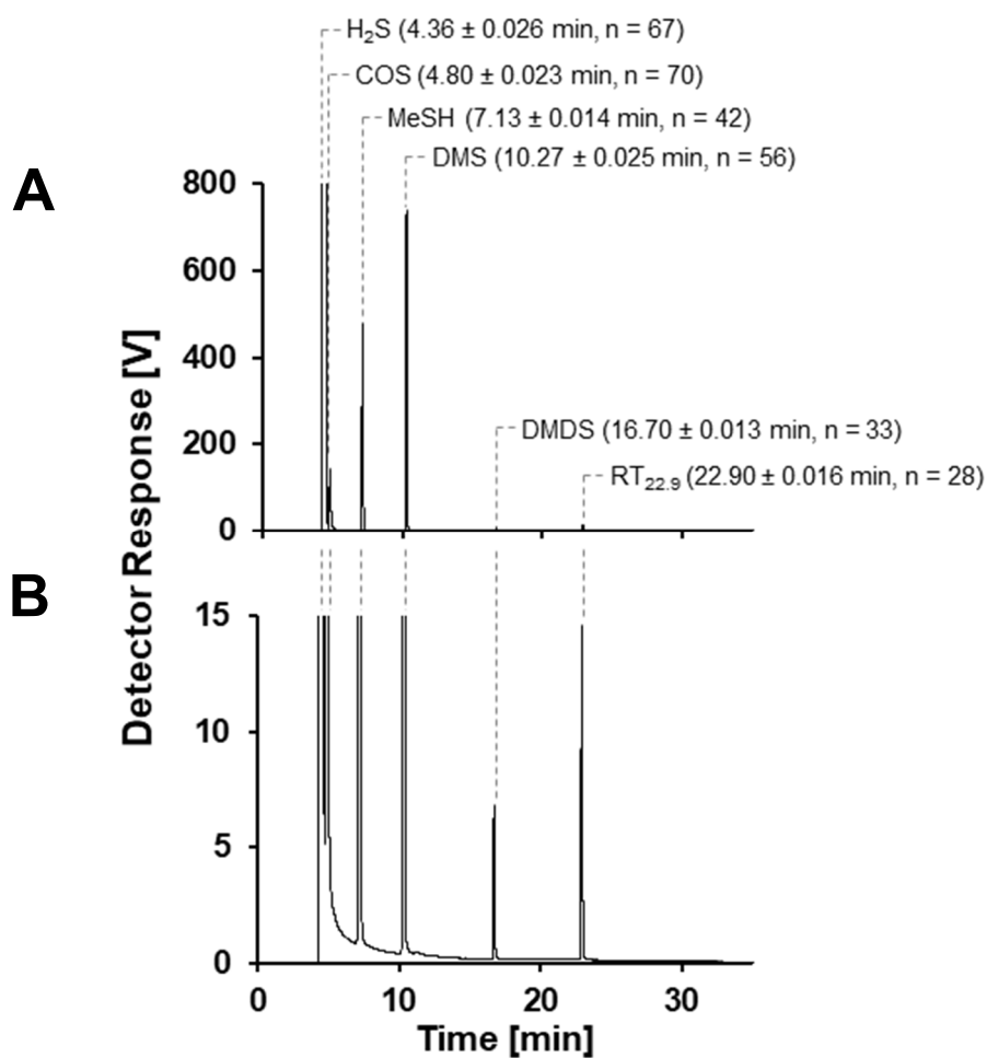
Supplementary Figure S1. Example chromatogram for day 14 of the seawater incubations with Ulva intestinalis . Panels A and B scaled to a detector response of 0-800 V and 0-15 V, respectively. Dashed lines indicate peak identities with retention times and sample sizes shown in brackets.
