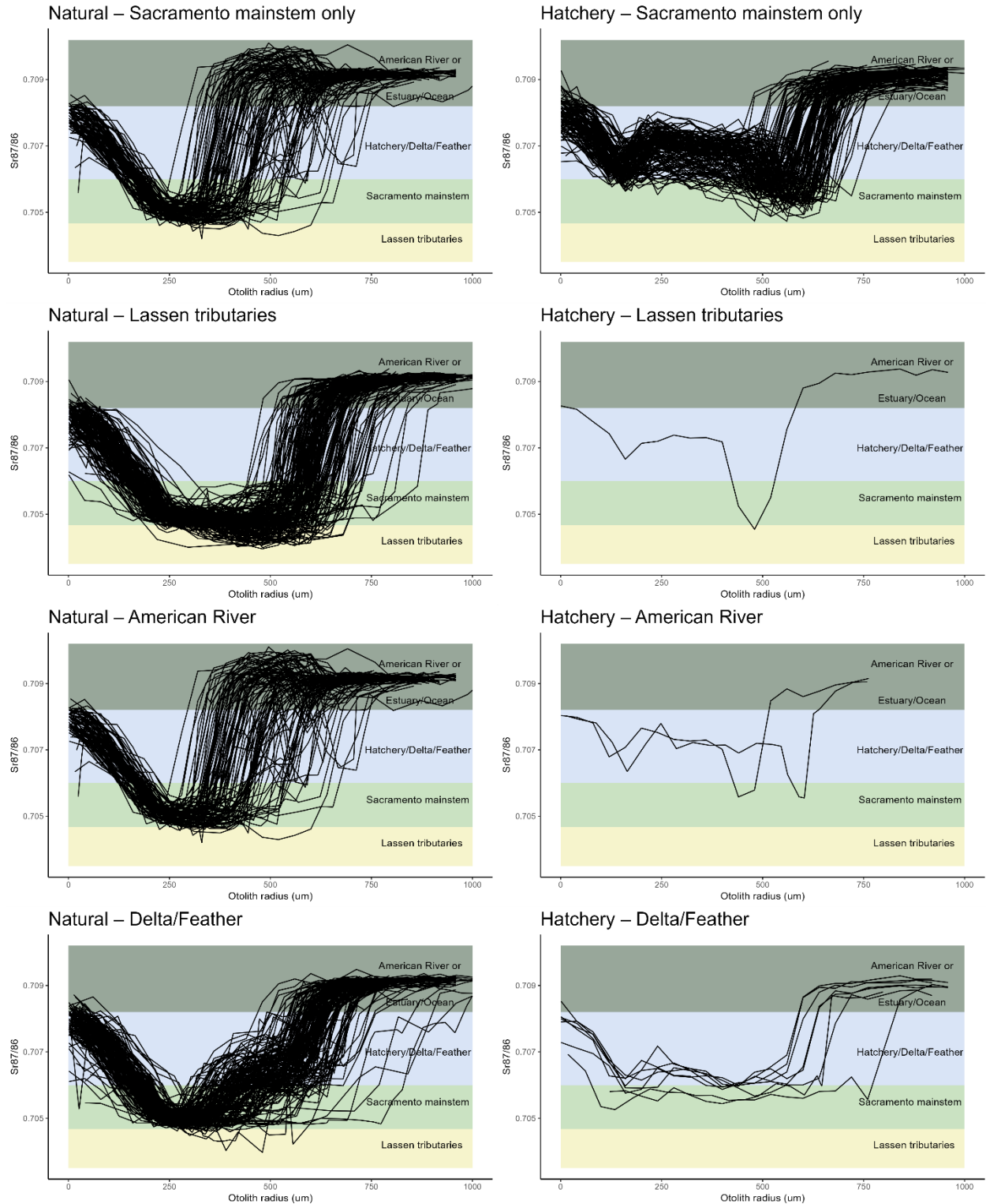
Supplemental Figure 2. Strontium isotopic ratio profiles of natural-origin (left) and hatchery-origin life histories (right) during their freshwater rearing and ocean entry phases.
