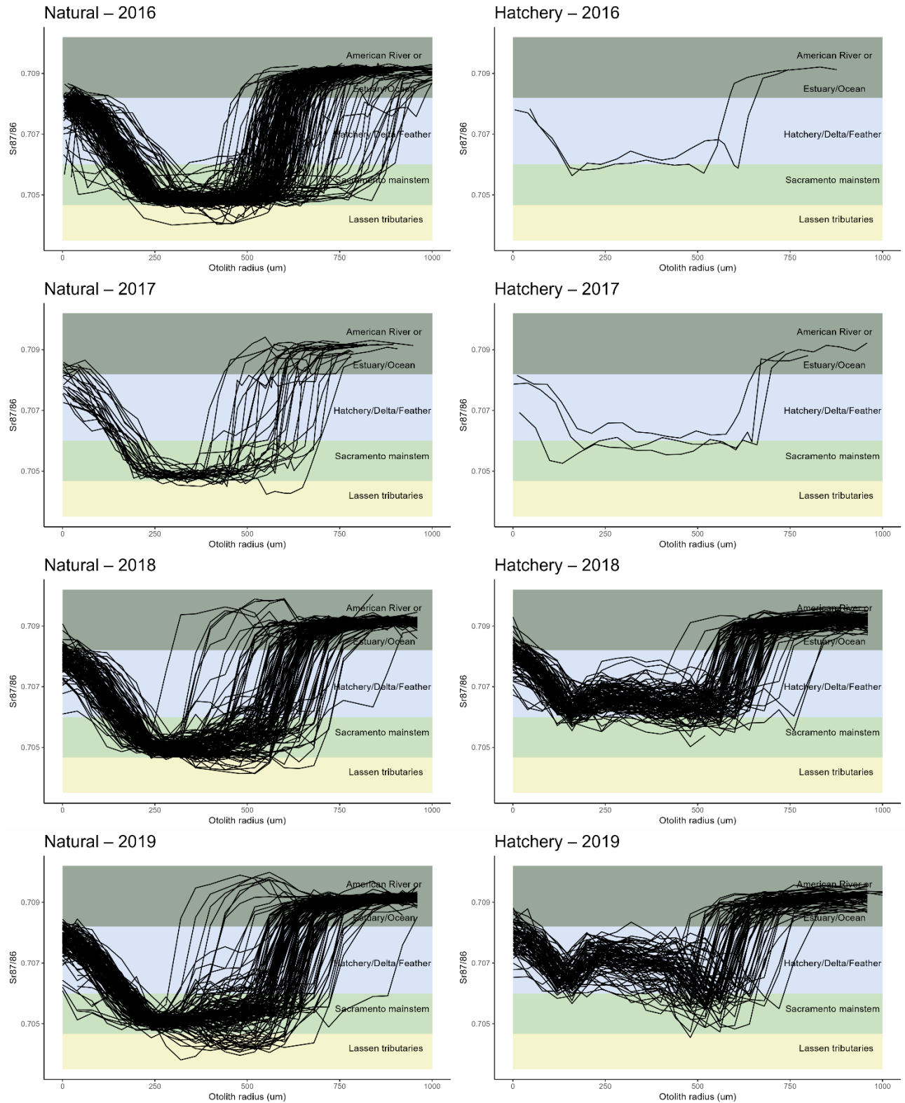
Supplemental Figure 1. Strontium isotope profiles for winter-run Chinook Salmon from 2007-2009 and 2015-2019 of natural- and hatchery-origin.
