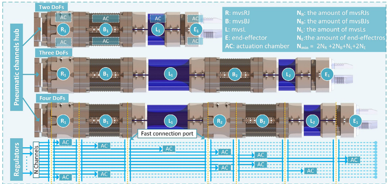
FIGURE 6 | Modular pneumatic routing and mechanical interface design. Each module (e.g., mvsBJ, mvsRJ, and mvsL) is equipped with a universal modular adapter featuring male and female ends of standardized diameter, enabling direct axial connection. Bolt–nut ports distributed around the interfaces ensure alignment and apply clamping force, compressing internal O-rings to seal the joint. All modules include 10 internal pneumatic channels (visualized as blue lines), allowing continuous airflow throughout the assembled co-bot regardless of configuration. A pneumatic hub at the base provides external tube connections via quick push-in fittings and passes the 10 channels upward through a male adapter for seamless integration. This architecture ensures both modularity and uninterrupted pressure routing across complex co-bot assemblies.
