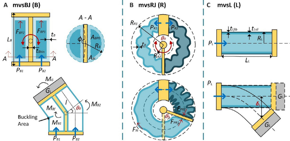
FIGURE 12 | Analytical actuation models and structural schematics of the three modular soft actuation units. (A) Schematic and modeling of the module mvsBJ. The mvsBJ consists of two internal chambers actuated antagonistically. A pressure difference \Delta P_B leads to asymmetric chamber deformation and results in a bending angle \theta_B . The extending chamber is reinforced with embedded fibers, producing primarily axial strain, modeled using the Mooney-Rivlin hyperelastic formulation. Resulting torques are computed from pressure and resistive forces, and a mapping function f_{\theta}^B(\Delta P_B) is derived under quasi-static equilibrium. (B) Schematic and force model of mvsRJ. This module shares similar material and chamber structure with mvsBJ but features a rotational output. The actuation forces from chambers with pressures P_{R1} and P_{R2} are balanced with resisting stress and a simplified constant frictional term. The rotational angle \theta_R is then mapped to pressure difference via f_{\theta}^R(\Delta P_R) . (C) Analytical model of the module mvsL, modeled as a fiber-constrained pressure-tunable cantilever beam. Internal pressure P_L increases the effective Young's modulus ( E_{Leff} ), enabling modulation of beam stiffness. Based on Euler–Bernoulli beam theory, the end deflection \delta_L under an external load G_L is expressed as a function of internal pressure.
