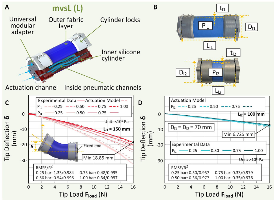
FIGURE 3 | Mechanical architecture and predictive tip deflection models for the modular variable-stiffness link (mvsL). (A) Detailed cross-sectional CAD rendering displaying the outer fabric layer, internal fluid channels, and nested silicone cylinder configurations. (B) Physical prototypes fabricated with distinct parameter constraints, delineating variations in active length ( L_1 ) and body diameter ( D_1 ). (C) Transverse tip deflection \delta plotted against a dynamic tip load spectrum ( F_{load} from 0 to 16 N) for the longer link prototype ( L_1 = 150 mm), providing a continuous overlay comparison between raw experimental metrics and the analytical actuation model predictions across multiple pressure thresholds ( P_{11} from 0.25 to 1.00 bar) along with the corresponding error matrix. (D) Quantitative tip deflection validation profiles for the shorter link variant ( L_2 = 100 mm) under identical loading boundaries, confirming tight model fitting accuracies with specific RMSE and R^2 correlation metrics annotated for each active pressure state.
