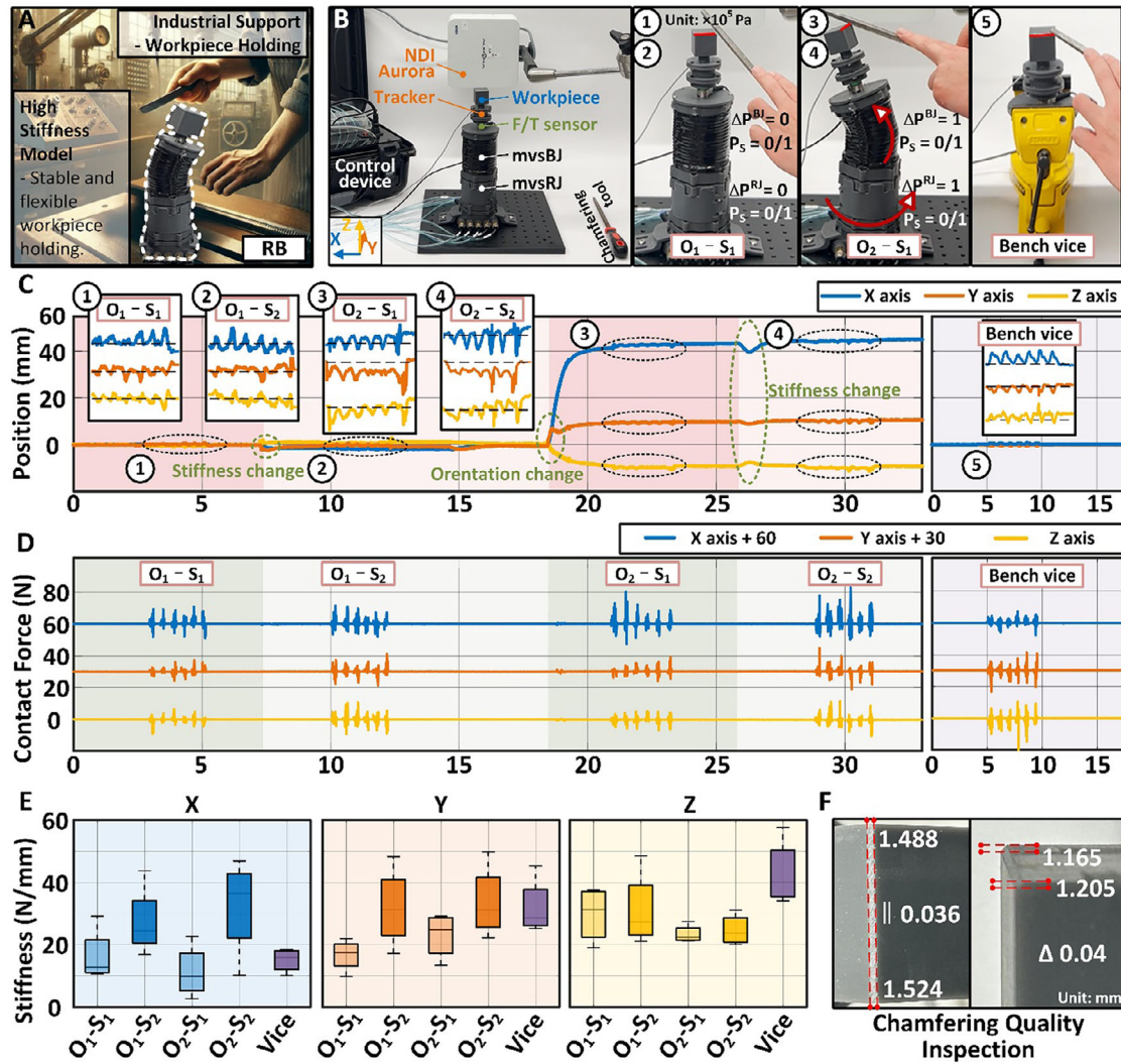
FIGURE 9 | Results of Industrial Manufacturing Support. (A) The co-bot with the RB configuration, setting as high stiffness model, holds a workpiece to support the worker to conduct the chamfering process. (B) The experimental setup for mimicking the support of the chamfering process, where the F/T sensor was mounted between the end of the mvsBJ and the holding mechanism of the workpiece, and the tracking sensor is mounted on the top of the F/T sensor to record the position change during the chamfering. In ①②, there are two different stiffness models in the same stand position. In ③④, there are two different stiffness models in the same bending position. In ⑤, there is the same setup mounted on a traditional bench vice for comparison purposes. (C) The recording of the position change of the workpiece in 5 situations. (D) The recording of the force from the force sensor in 5 situations. (E) The stiffness result calculated by the recorded position change and force. (F) The quality inspection of the chamfer after we finished the chamfering process on the co-bot.
