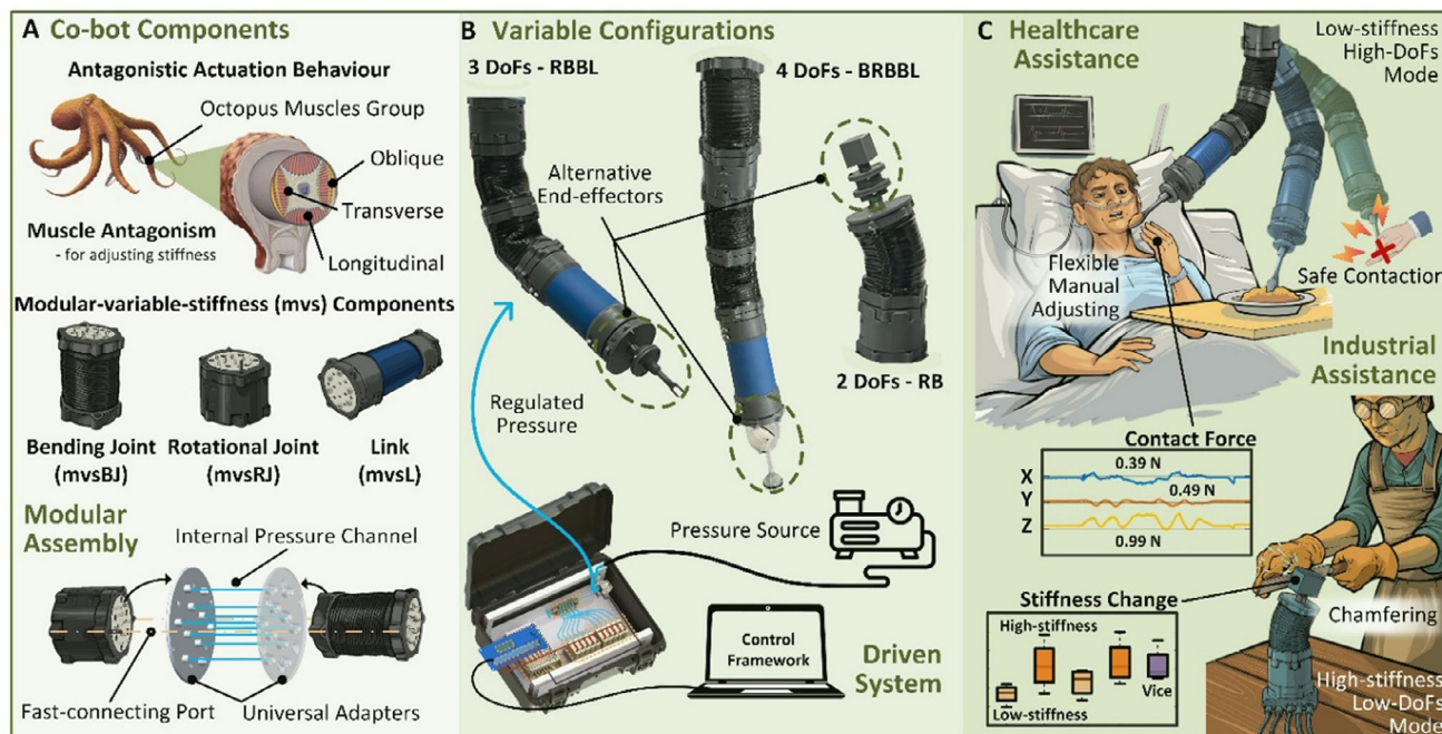
FIGURE 1 | Introduction of the modular variable stiffness co-bot system. (A) Bio-inspiration from octopus muscle groups exhibiting antagonistic actuation for variable stiffness control. This principle is adopted in the design of modular variable stiffness (mvs) co-bot components, including the bending joint (mvsBJ), rotational joint (mvsRJ), and link (mvsL). The components can be rapidly assembled into various co-bot configurations through universal adapters, integrated pressure channels, and quick-connect ports. (B) By selecting different types and numbers of components, modular variable stiffness co-bots with 2-, 3-, and 4-DoF configurations can be assembled and equipped with alternative end-effectors to meet diverse task requirements. A unified actuation system, comprising the control framework and pressure regulation unit, enables consistent control across all co-bot configurations. (C) Two application scenarios—healthcare and industrial assistance—were conducted to demonstrate the flexibility and safety of the proposed co-bot system. In the healthcare assistance scenario, a 3-DoF co-bot was employed to deliver food from the table to a position near the patient's mouth. The patient could then manually adjust the end-effector to bring the food to their mouth with minimal effort, as the co-bot operated in a low-stiffness mode. The recorded contact forces indicated that the average force along all three axes was less than 1 N, confirming the system's safety during human interaction. In the industrial assistance scenario, a 2-DoF co-bot was used to hold a workpiece, providing a flexible yet stable working position under a high-stiffness mode. The measured holding stiffness demonstrated that the proposed antagonistic stiffness adjustment method significantly enhanced the overall rigidity of the co-bot, reaching a stiffness level comparable to that of a conventional workbench.
