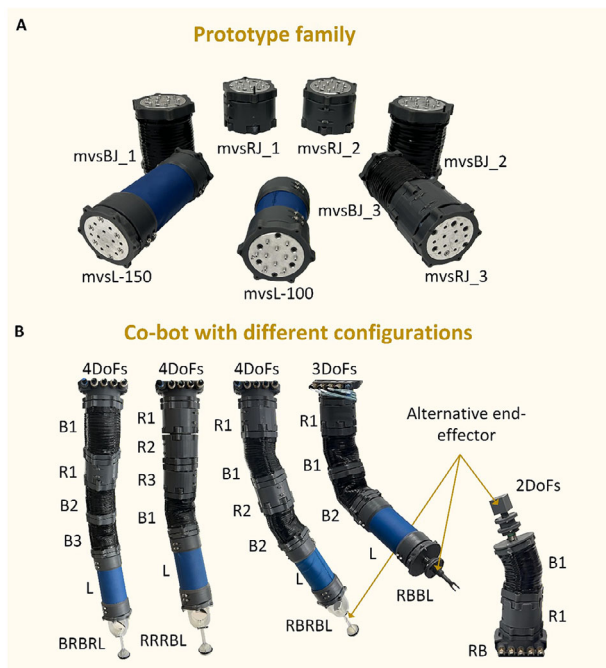
FIGURE 5 | Comprehensive component ecosystem and multi-DoF architectural configurations of the customizable co-bot platform. (A) The complete hardware prototype family, showcasing the fabricated modules with varied specifications and geometric boundaries (including mvsBJ, mvsRJ, and mvsL series). (B) Demonstrations of five representative reconfigurable co-bot topologies assembled via universal modular adapters, spanning distinct degrees of freedom (from a highly agile 4-DoF arm down to a compact 2-DoF system) equipped with alternative customized end-effectors for safety-oriented automation tasks.
