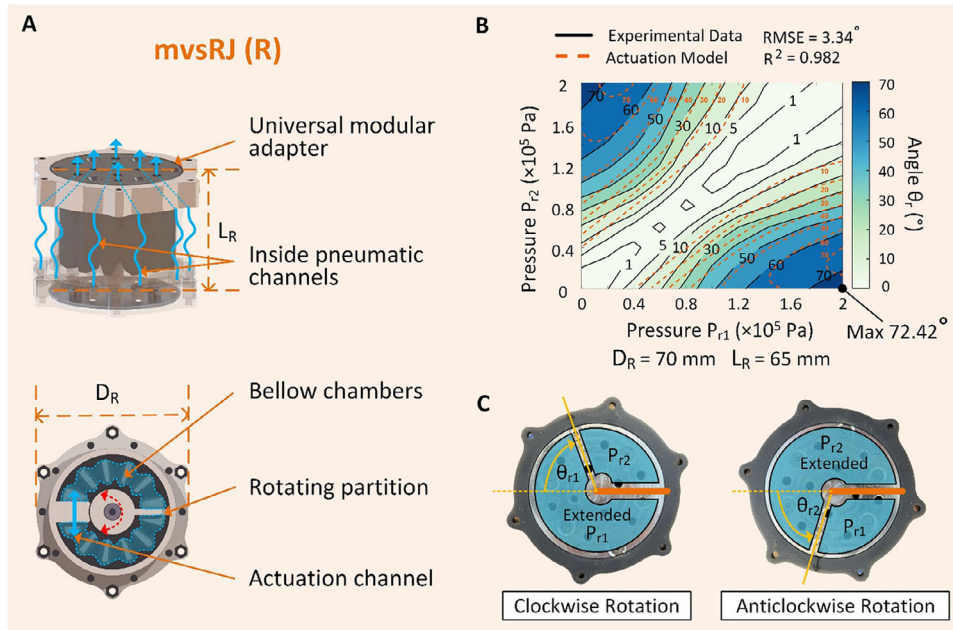
FIGURE 4 | Layout configuration and angular mapping models of the modular variable-stiffness rotational joint (mvsRJ). (A) Exploded CAD view and internal radial cross-section highlighting the layout of the multi-segment internal bellow chambers, rotating partition wall, and modular universal adapters. (B) Integrated bi-directional rotation angle ( \theta_r ) response mapping contour under varied multi-channel pneumatic inputs ( P_1 and P_2 ), verifying a high predictive convergence between the empirical measurements (solid contour lines) and the proposed analytical actuation model (dashed orange contours) with a bounded global RMSE of 3.34° and an R^2 of 0.982. (C) Physical actuation prototypes displaying explicit clockwise and anticlockwise angular deflections under differential pressure expansion.
