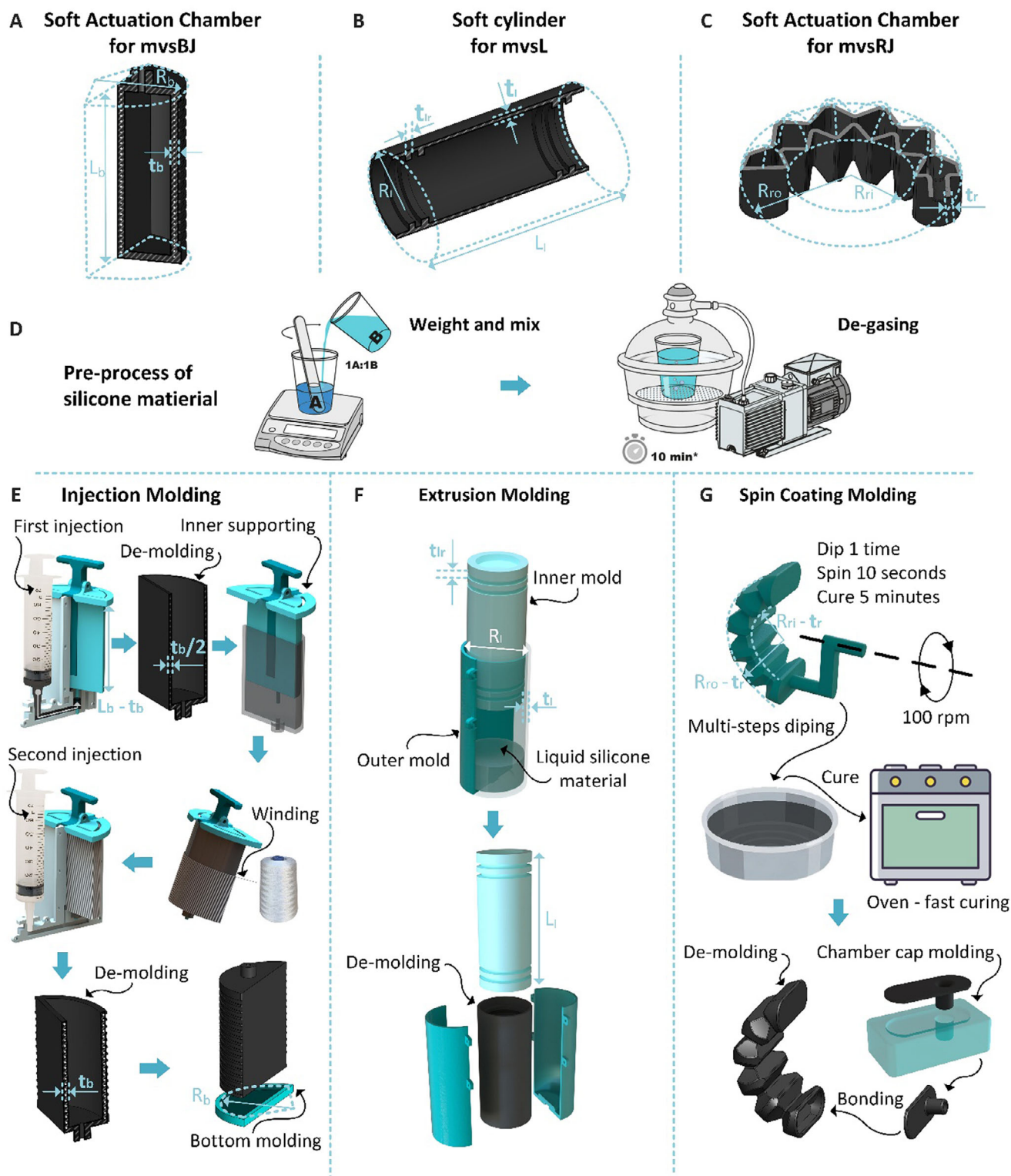
FIGURE 10 | The fabrication process of three key soft parts in each co-bot components. (A) The structure indication of the mvsBJ soft actuation chamber. (B) The structure indication of the mvsL soft cylinder. (C) The structure indication of the mvsRJ soft actuation chamber. (D) The common pre-process of the silicone material. (E) The injection molding process of mvsBJ actuation chamber. (F) The extrusion molding process of mvsL cylinder. (G) The spin coating molding process of mvsRJ actuation chamber.
