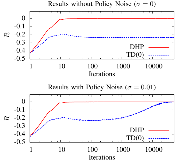
Fig. 1. Algorithm performances on the test problem using a neural network based actor critic architecture, as described in section IV-H; both with and without policy noise. The y axis shows the total total discounted long term reward, R . Compared to TD(0), the DHP method works well in the absence of stochastic exploration, and quickly attains optimal behaviour ( R = 0 ). The TD(0) method fails without stochastic exploration here (in fact it converges to a sub-optimal policy), but does learn slowly and successfully in the presence of policy noise.
